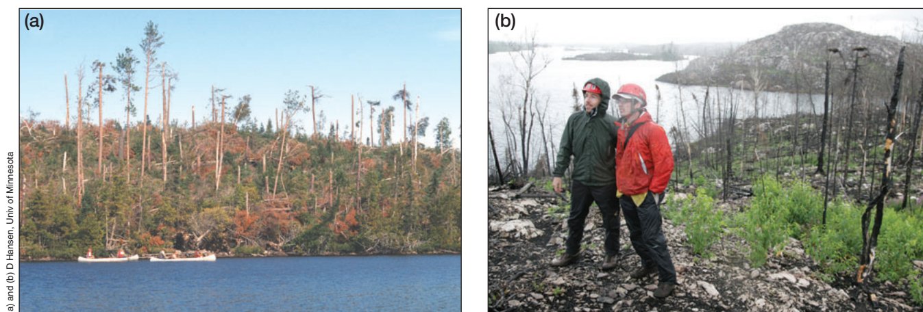
Figure 3. Major disturbance events will be more common with global warming and transform the composition of large tracts of forest. (a) Unlogged 200-year boreal forest with upper canopy destroyed by the derecho of 4 Jul 1999, Boundary Waters Canoe Area Wilderness, Minnesota. (b) The same forest as in (a), one year after the exceptionally severe Cavity Lake Fire of 2006, illustrating the combined impact of severe wind and fire disturbance.
